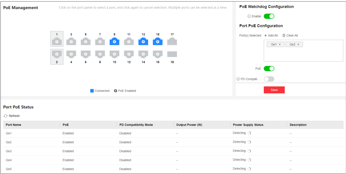
Figure 4-13 Configure PoE
